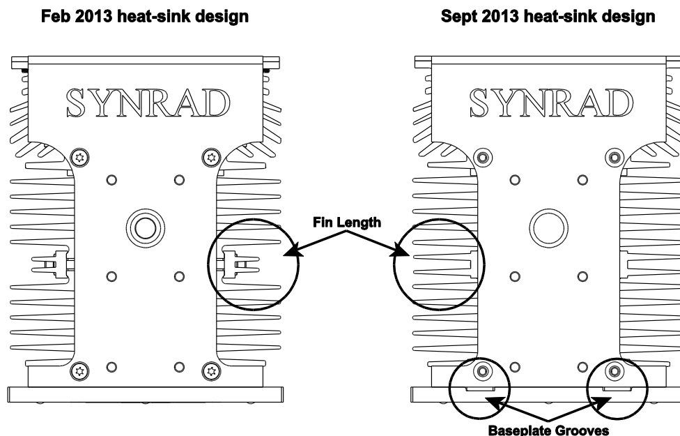
Figure 1 – Old (left) and new (right) split heat-sink designs
