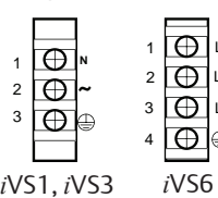
Figure 1. AC Input
